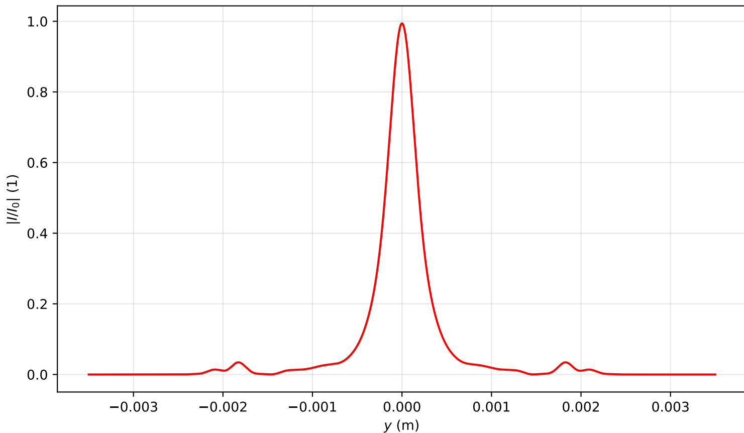
Intensity profile I(x=0, y, z=3.582)/I_0 , P_{in}=3.5P_{cr} , artificial time
